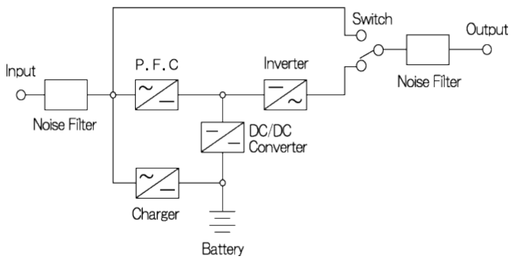
ALS-RM series block diagram
